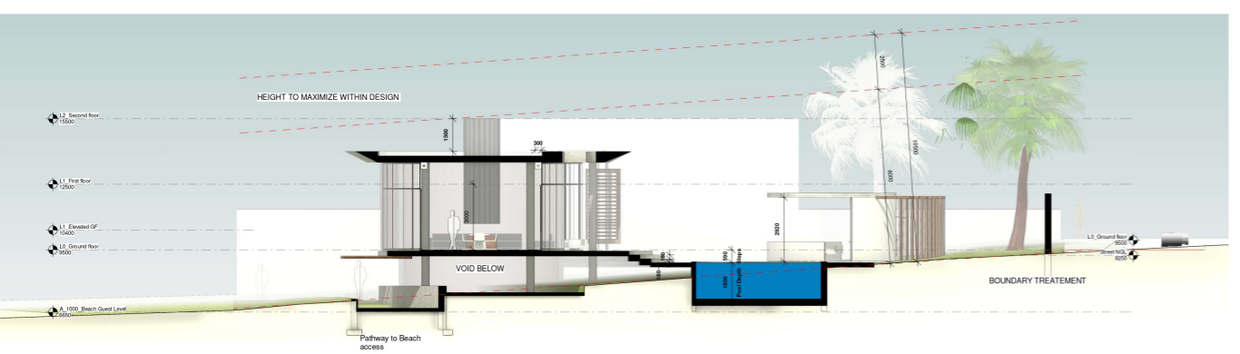
AA A 3000 SECTION AA 1:100
