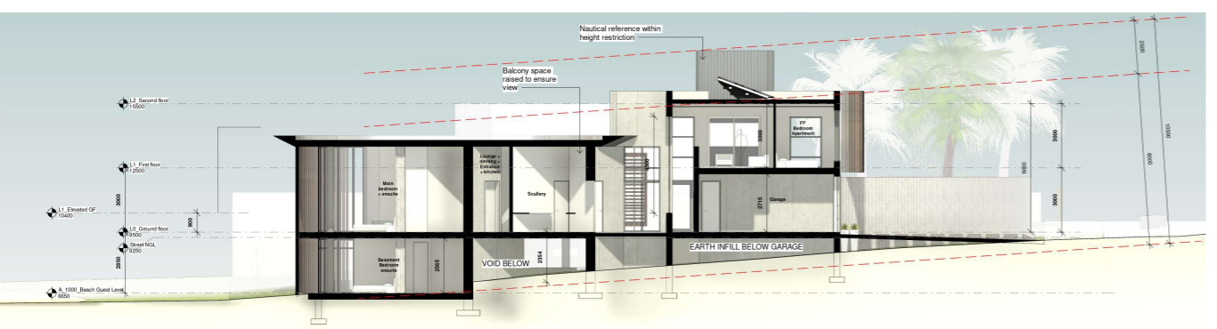
BB A 3000 SECTION BB 1:100
